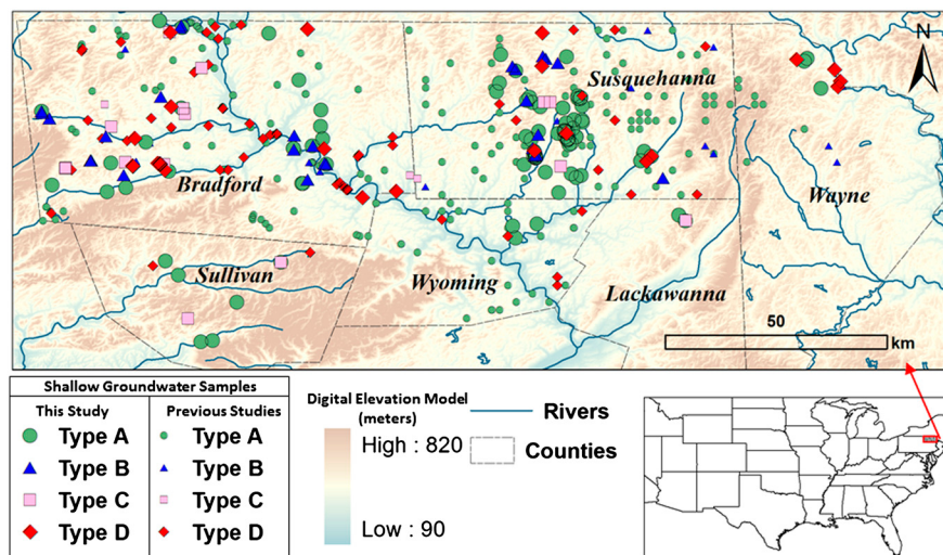
Fig. 1. Digital elevation model (DEM) map of northeastern PA. Shaded brown areas indicate higher elevations and blue-green shaded areas indicate lower elevations (valleys). The distribution of shallow (<90 m) groundwater samples from this study and previous studies (18, 19) are labeled based on water type. Two low salinity ( Cl < 20 mg/L) water types dominated by Ca-HCO_3 (type A = green circles) or Na-HCO_3 (type B = blue triangles) were the most common, and two higher salinity ( Cl > 20 mg/L) water types were also observed: Br/Cl < 0.001 (type C = pink squares) and brine-type groundwater Br/Cl > 0.001 (type D = red diamonds). Type D groundwater samples appear associated with valleys (Table S1) and are sourced from conservative mixing between a brine and fresh meteoric water. The DEM data were obtained from NASA's Shuttle Radar Topography Mission http://srtm.usgs.gov/ .
