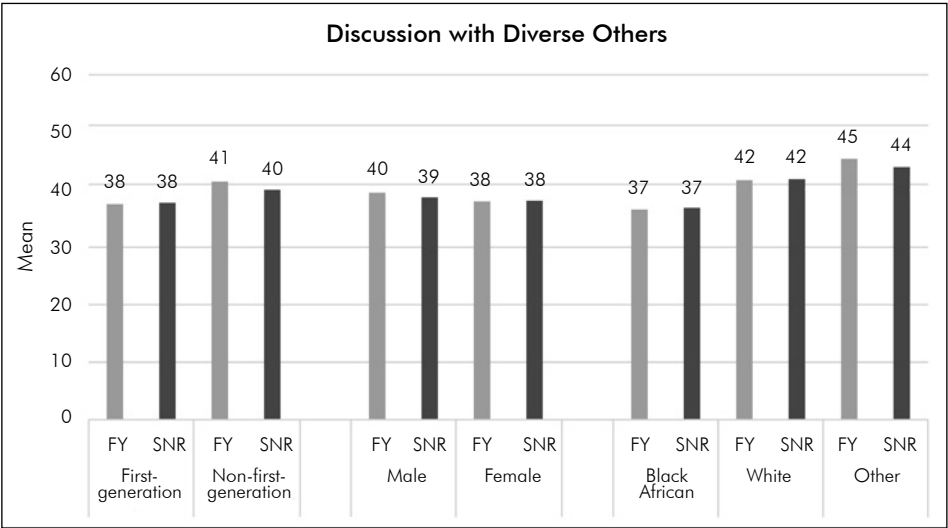
FIGURE 2.8 Discussion with Diverse Others mean scores for first-year and senior students by first-generational status, gender and race
