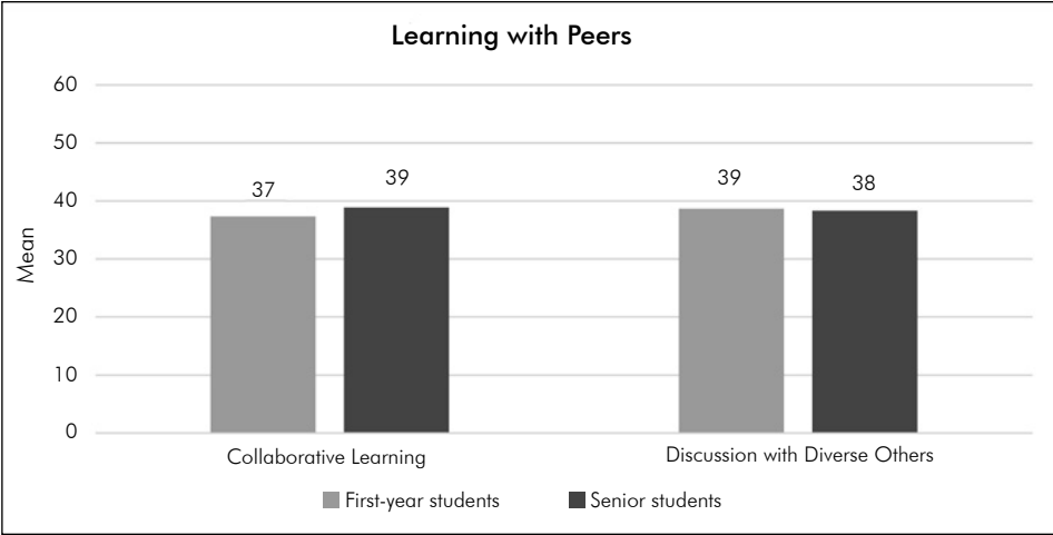
FIGURE 2.6 Learning with Peers engagement indicator mean scores for first-year and senior students
